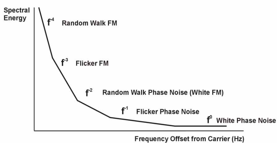
Figure 5-7 Typical Phase Noise Distribution
